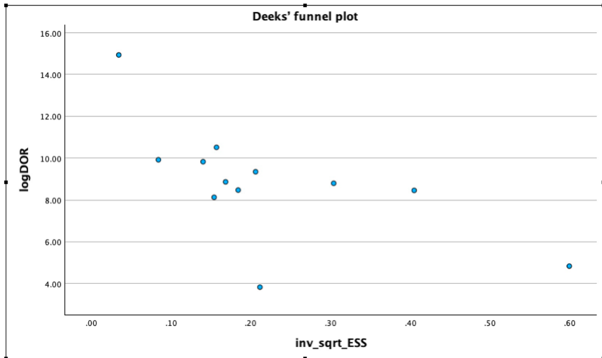
Supplementary Figure 1. Deek's funnel plot evaluating publication bias.
