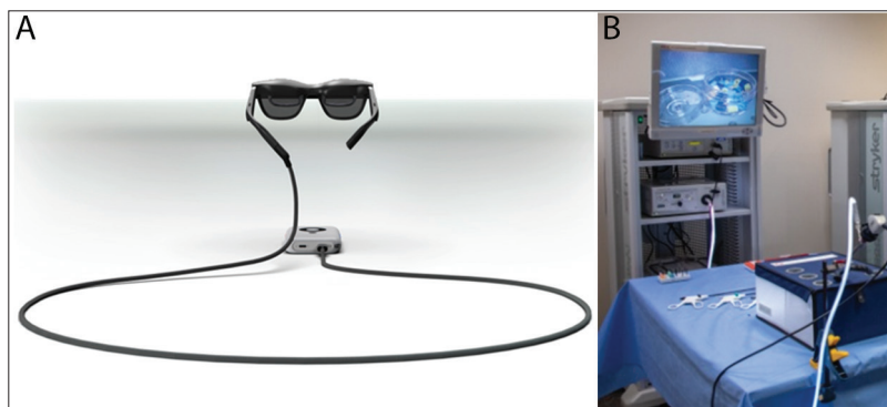
Figure 1. (A) XREAL Air 2 Ultra AR glasses. (B) Laparoscopic simulation setup with Stryker 30-inch laparoscopic monitor.
