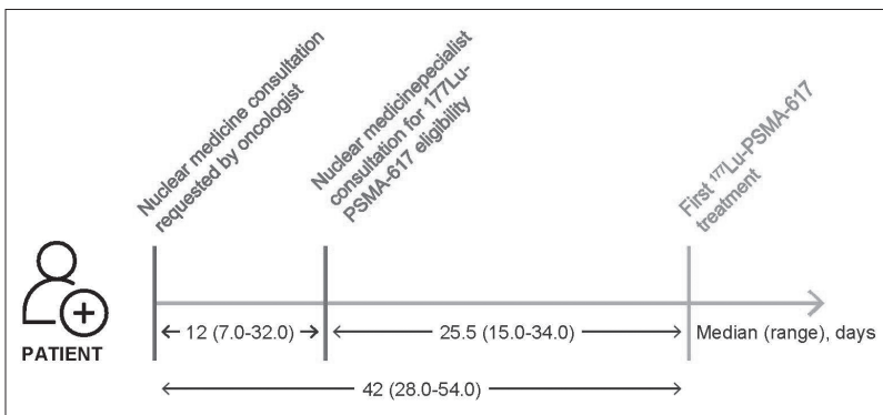
Figure 2. Time from oncology consultation to nuclear medicine consultation and treatment 177 Lu: lutetium-177; CT: computed tomography; FDG: fluorodeoxyglucose; PSMA: prostate-specific membrane antigen.
