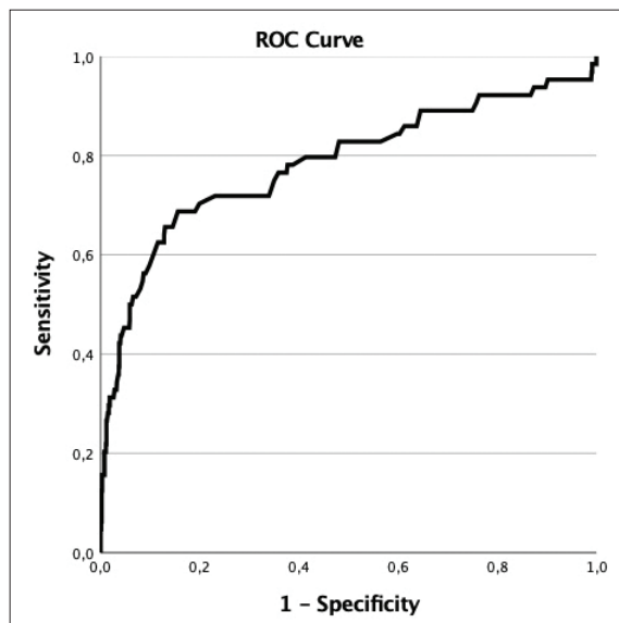
Figure 2. Receiver operating curve (ROC) illustrating the predictive value of renal pelvis urine density (RPUD) for postoperative infectious complications following semi-rigid ureterorenoscopy (area under the curve 0.784, 95% confidence interval 0.711–0.857, p < 0.001 ).
