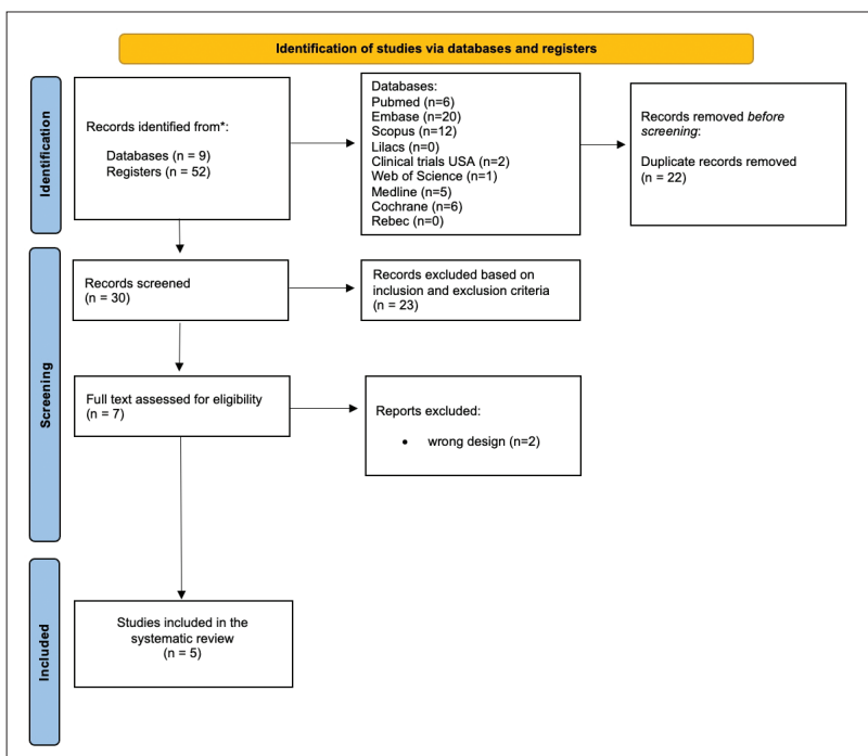
Figure 1. Prisma diagram.
