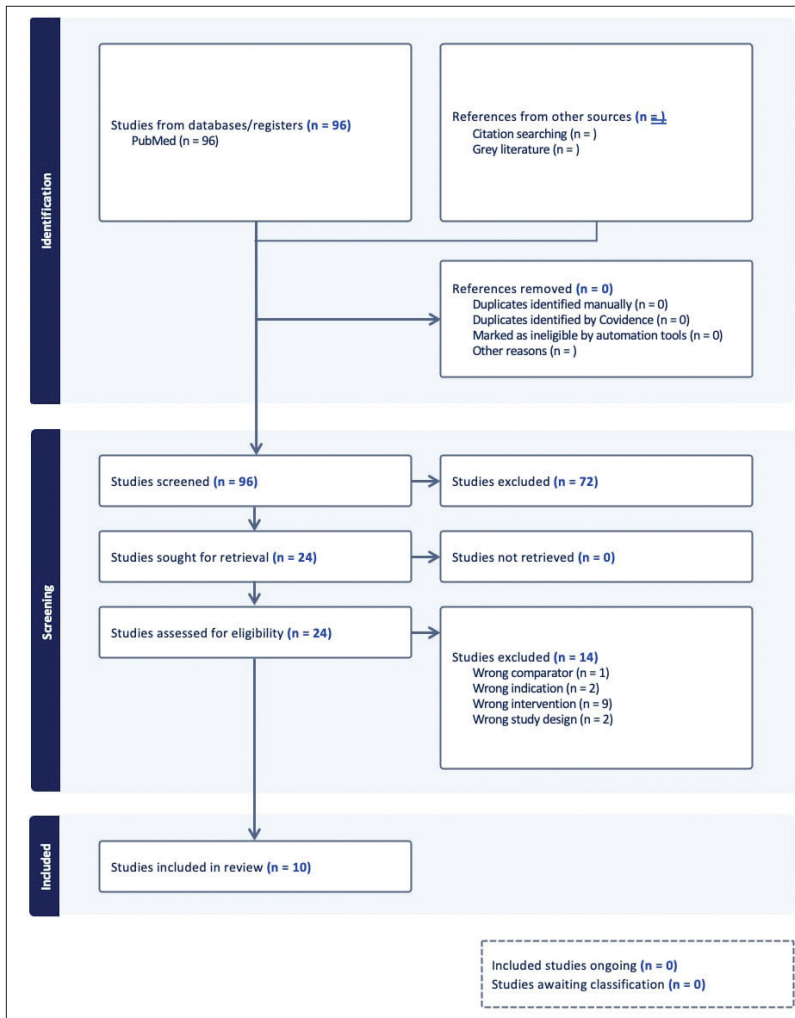
Figure 1. PRISMA flowchart.
