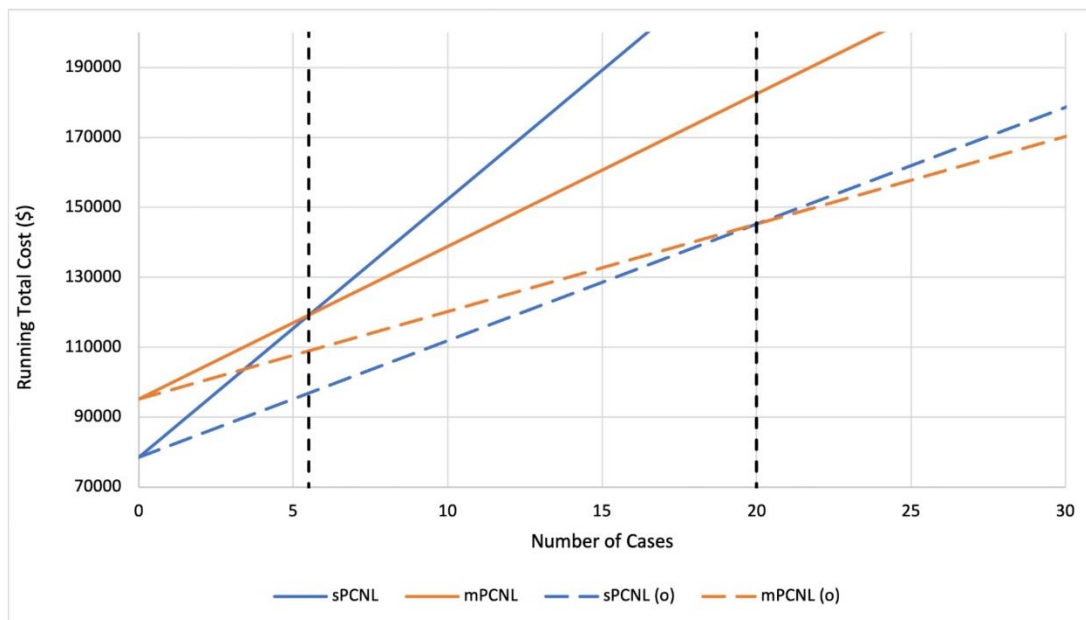
Figure 2. Cost-per-case regression of total running costs comparison between standard percutaneous nephrolithotomy (sPCNL) and mini (m)PCNL intersects at 5.51 cases, and at 20 cases when eliminating hospitalization costs (only operative costs).
