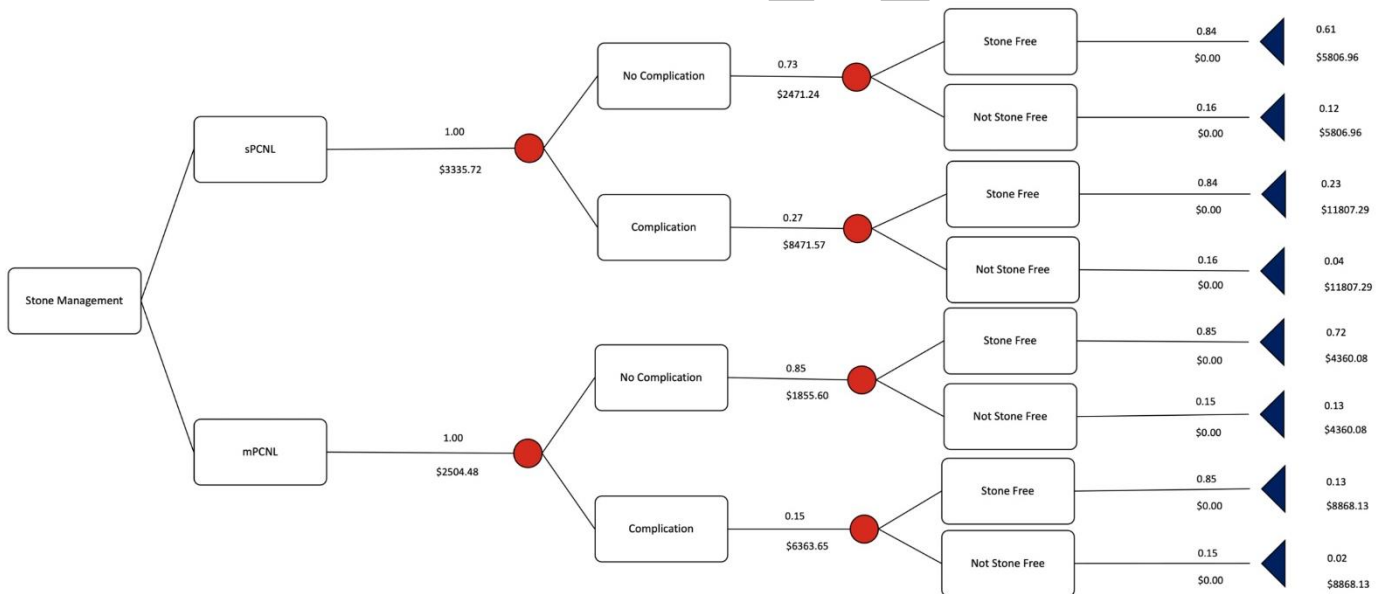
Figure 1. Decision tree model comparing outcomes between percutaneous nephrolithotomy (PCNL) and mini (m)PCNL. The decision tree starts with the option of stone management with PCNL or mPCNL. Circles represent chance nodes with possible events. Top values are the probability of the event occurring, with the bottom value representing the cost of that event occurring. End points (triangles), have final cumulative probabilities and costs of occurring, represented by the top and bottom values respectively. Probability of a pathway = summated probability of all events in the pathway. Cost of a pathway = the sum of the cost of all events in the pathway.
