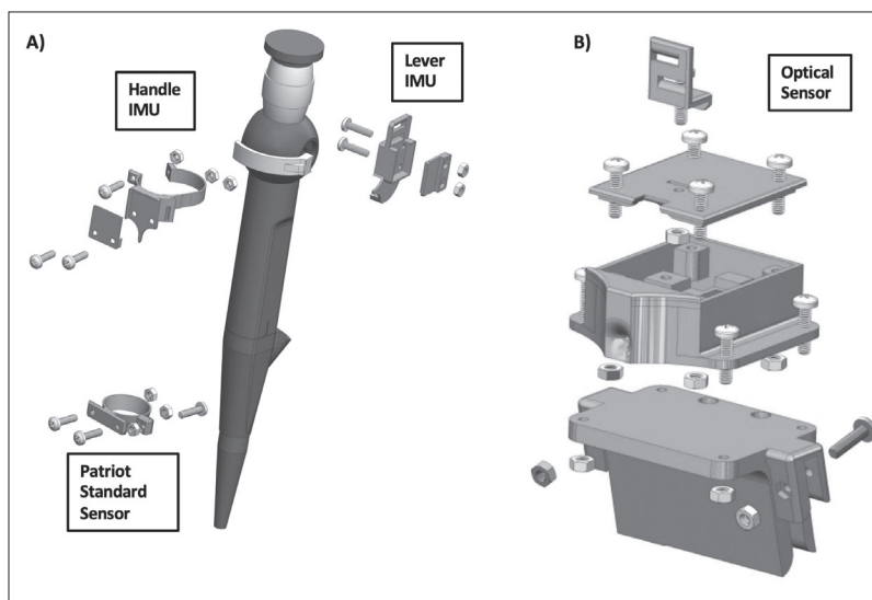
Figure 4. Diagrams of sensor mounts and components used in the motion-tracking system. (A) Mounts for two internal measurement units and Patriot sensor used on the ureterscope. (B) Attachment clip (bottom) and the housing (center) for the optical sensor.
