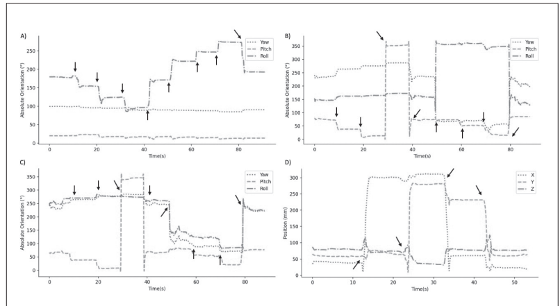
Figure 6. Position and absolute orientation data collected from the Polhemus Patriot sensor attached to the ureteroscope handle. Orientation data when rotating ureteroscope (A) in the z-axis (roll); (B) in the y-axis (pitch) from 5 – 365 degrees; (C) in the x-axis (yaw). (D) Position data when translating scope 300 mm along the x-axis (+), y-axis (+), x-axis (–), and y-axis (–) every 10 seconds.
