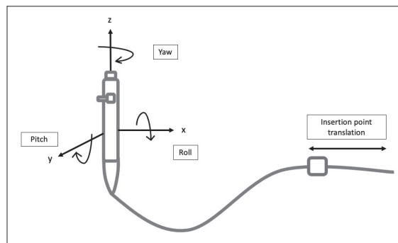
Figure 3. Illustration of the measurement of roll, pitch, and yaw in relation to the rotational movement of the ureteroscope and translation at the insertion point.
