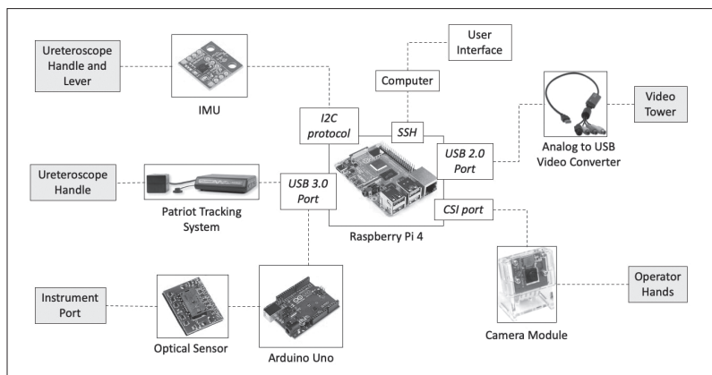
Figure 1. Diagram of connections between Raspberry Pi 4 and all system peripherals. The Pi has USB 2.0 and 3.0 ports, inter-Integrated Circuit (I2C) communication protocols, and a Camera Serial Interface (CSI) camera port. The Pi is controlled by the user remotely through a personal computer with Secure Shell Protocol (SSH).
