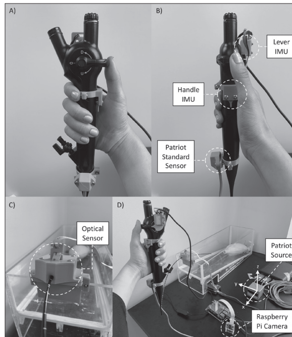
Figure 2. Complete motion-tracking and video-capture tool. (A) (B) Inertial measurement unit and Patriot standard sensor fitted onto the single-use flexible ureteroscope. (C) Optical sensor fitted to project above the insertion point of the ureteroscope onto a simulator box. (D) Complete view of tool with Patriot source (i.e., reference coordinates for x-, y-, and z-axes) and Raspberry Pi camera module pointing toward operator's hands.
