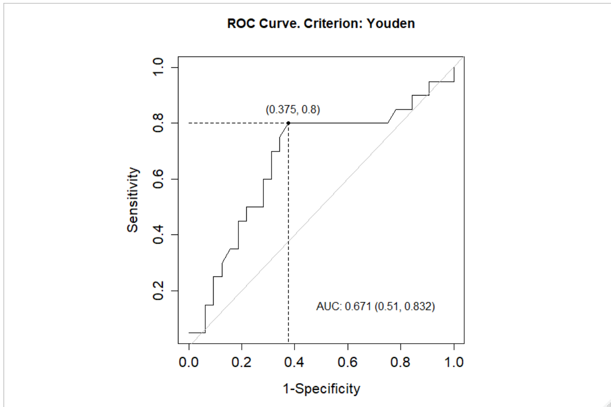
Supplementary Figure 1 Receiver operator curve for ellipsoid area as a predictor of biopsy positivity.
