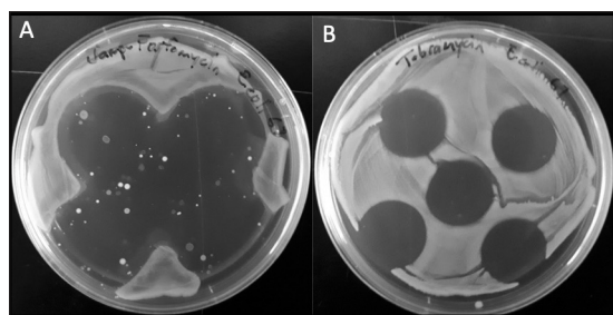
Fig. 1. Fosfomycin at the concentration tested was effective at inhibiting the growth of E. coli 67 with a zone of inhibition that was similar to that of tobramycin. Results of fosfomycin are shown in panel A, and tobramycin in panel B.
