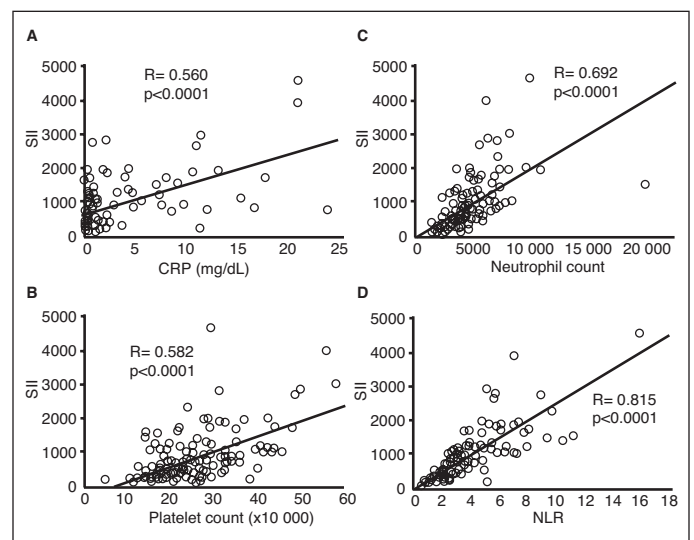
Fig. 1. Correlation between systemic immune inflammation index (SII) and other inflammatory parameters, including (A) C-reactive protein (CRP); (B) platelet count; (C) neutrophil count; and (D) neutrophil-to-lymphocyte ratio (NLR).
