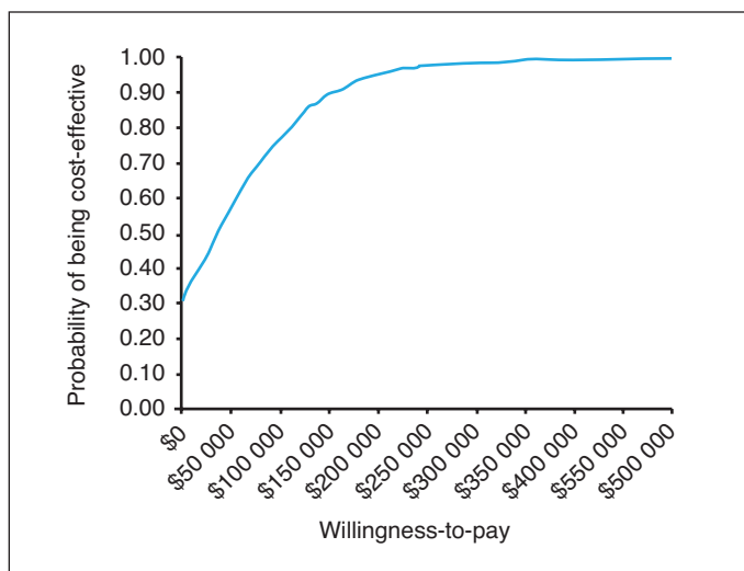
Fig. 2. Cost-effectiveness acceptability curve (CEAC).
