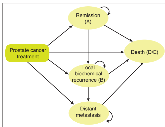
Fig. 1. Diagrammatic representation of the Markov model. States of the model is represented by the ovals, transition between states represented by the arrows.
